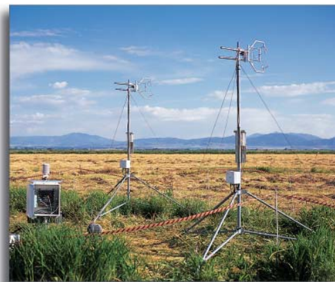
Eddy covariance experiments over marsh grass (Cache Valley, UT).
